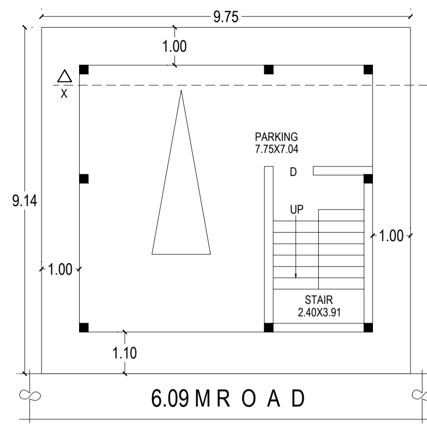
STILT FLOOR
