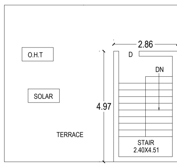
TERRACE FLOOR
